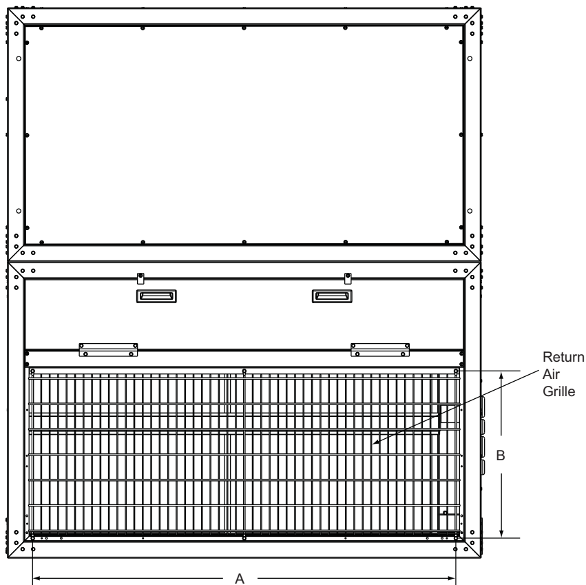
FIGURE 1 - RETURN AIR GRILLE ACCESSORY
