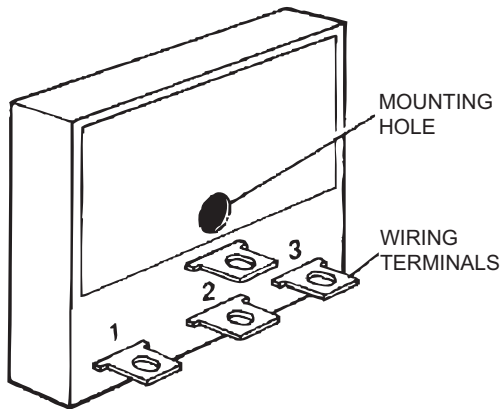
Figure 1: TIMER CONTROL
