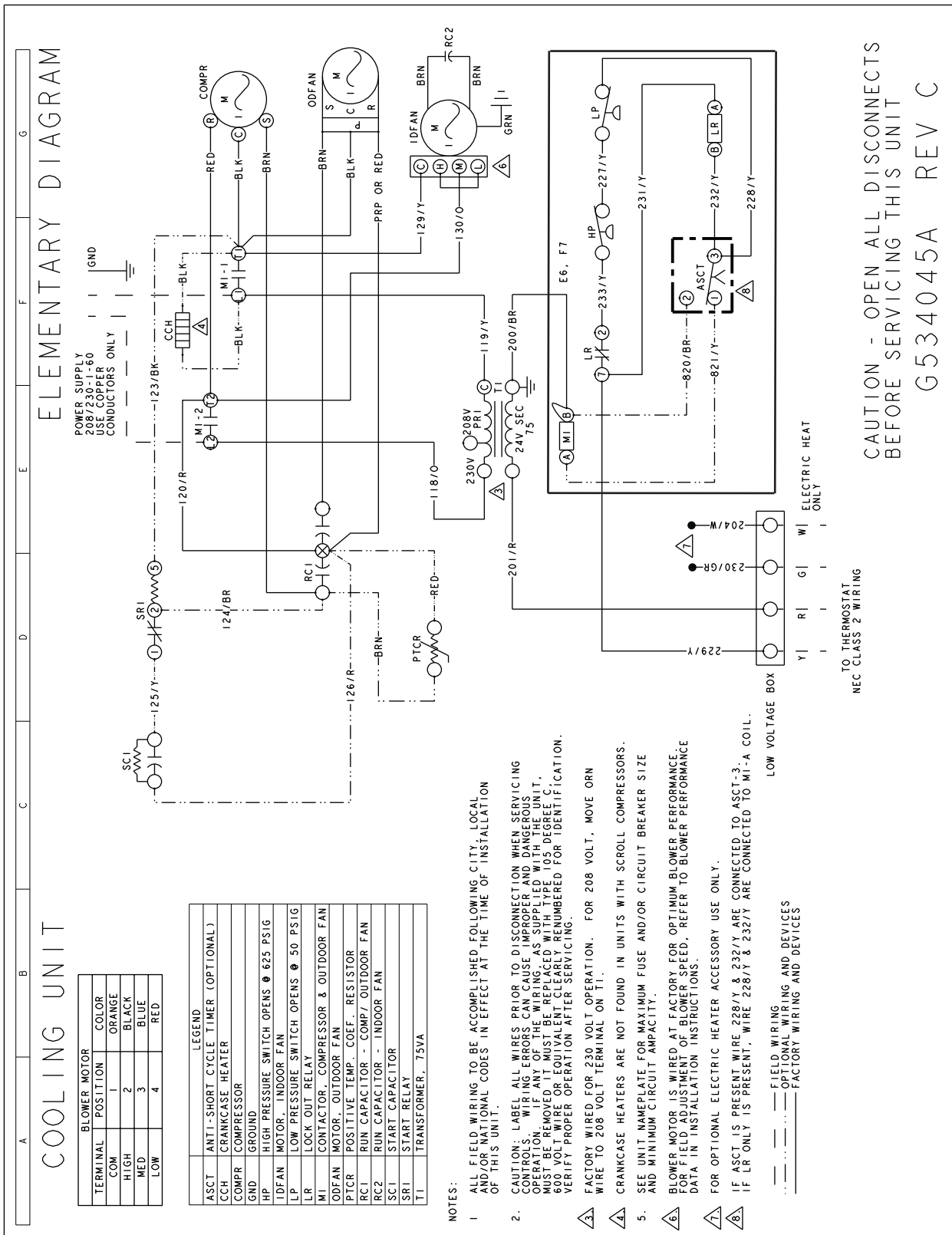
Figure 2: Typical Anti-Recycle Timer Kit Wiring Diagram
