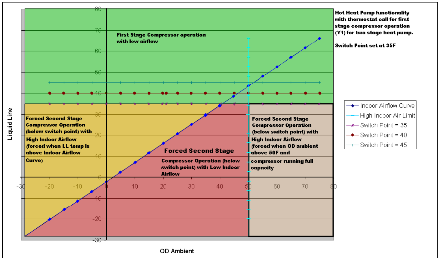
FIGURE 4: Hot Heat Pump Indoor Airflow Control and Forced Second Stage
