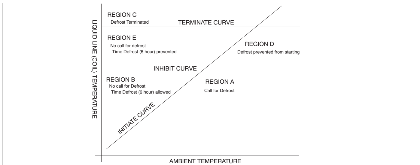
FIGURE 3: Defrost Operation Curves
