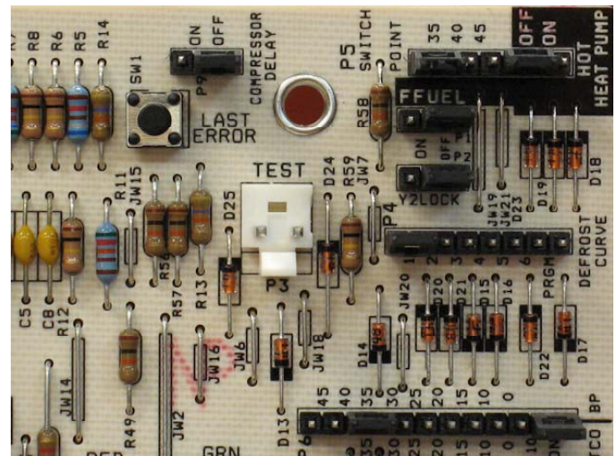
FIGURE 2: Jumper Inputs
