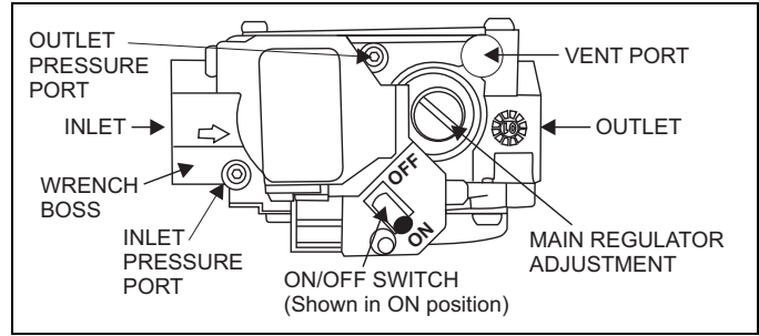
FIGURE 2: Single Stage Gas Valve
