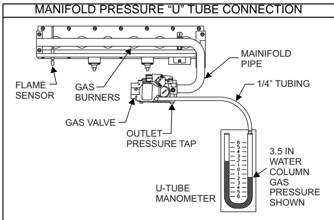
FIGURE 4: Reading Gas Pressure - 95% 33" Models
