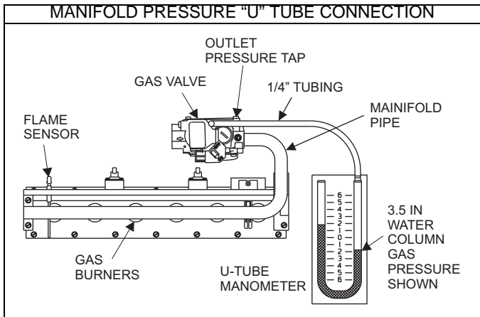
FIGURE 3: Reading Gas Pressure - 80% 33" Models
