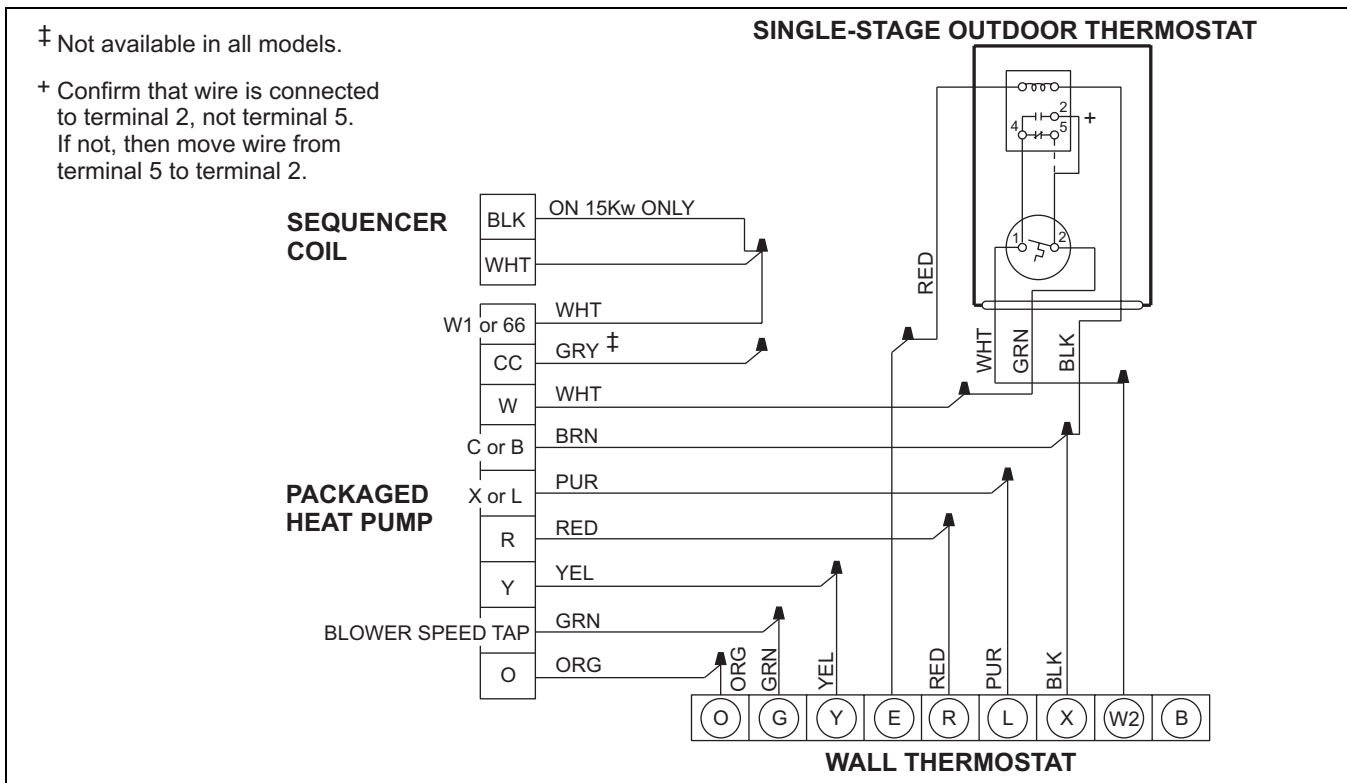
FIGURE 5: Wiring Connections for JP/PHP Packaged Heat Pump with Single Stage Outdoor Thermostat
