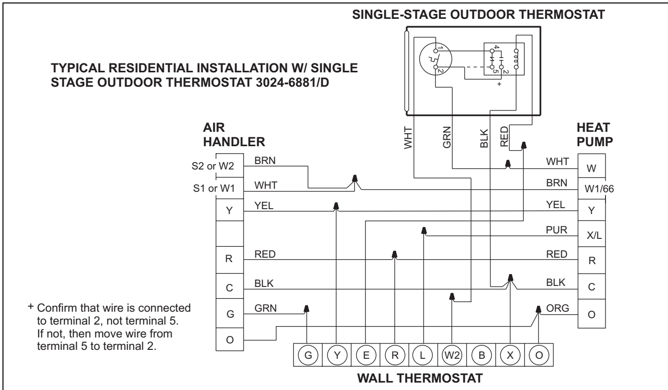
FIGURE 1: Wiring Connections for Typical Residential Installation with Single Stage Outdoor Thermostat
