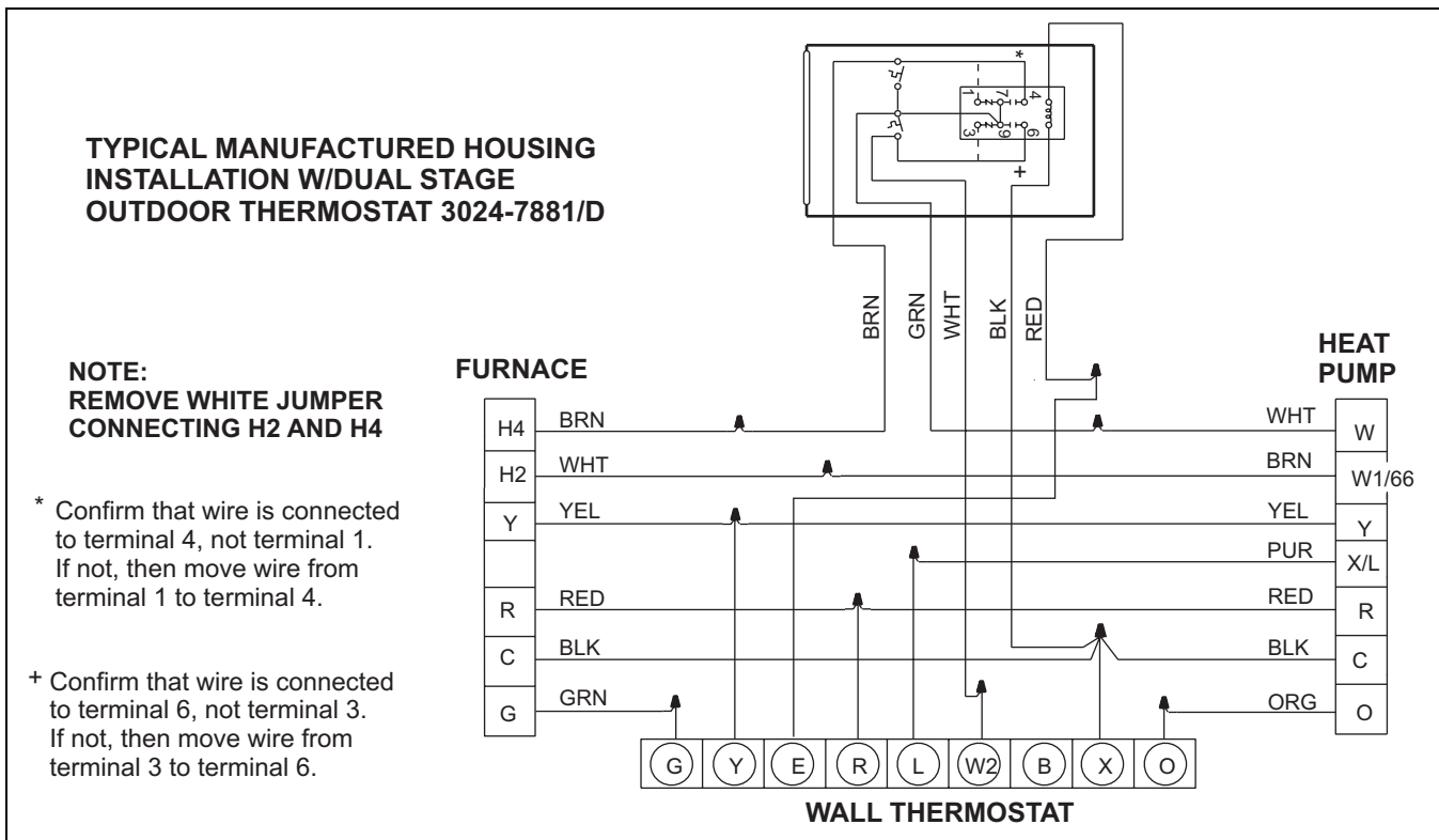
FIGURE 4: Wiring Connections for Typical Manufactured Housing Installation with Dual Stage Outdoor Thermostat
