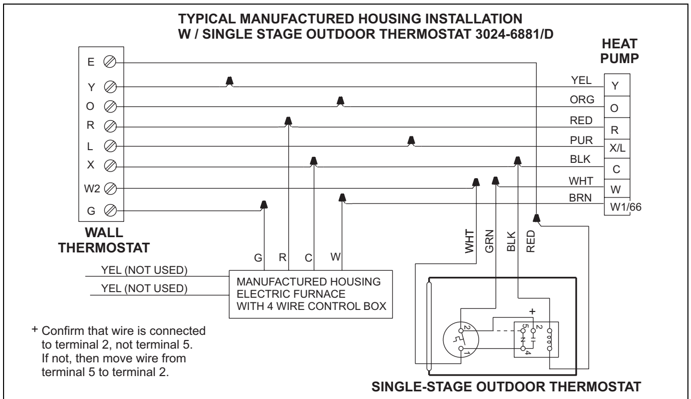
FIGURE 3: Wiring Connections for Typical Manufactured Housing Installation with Single Stage Outdoor Thermostat
