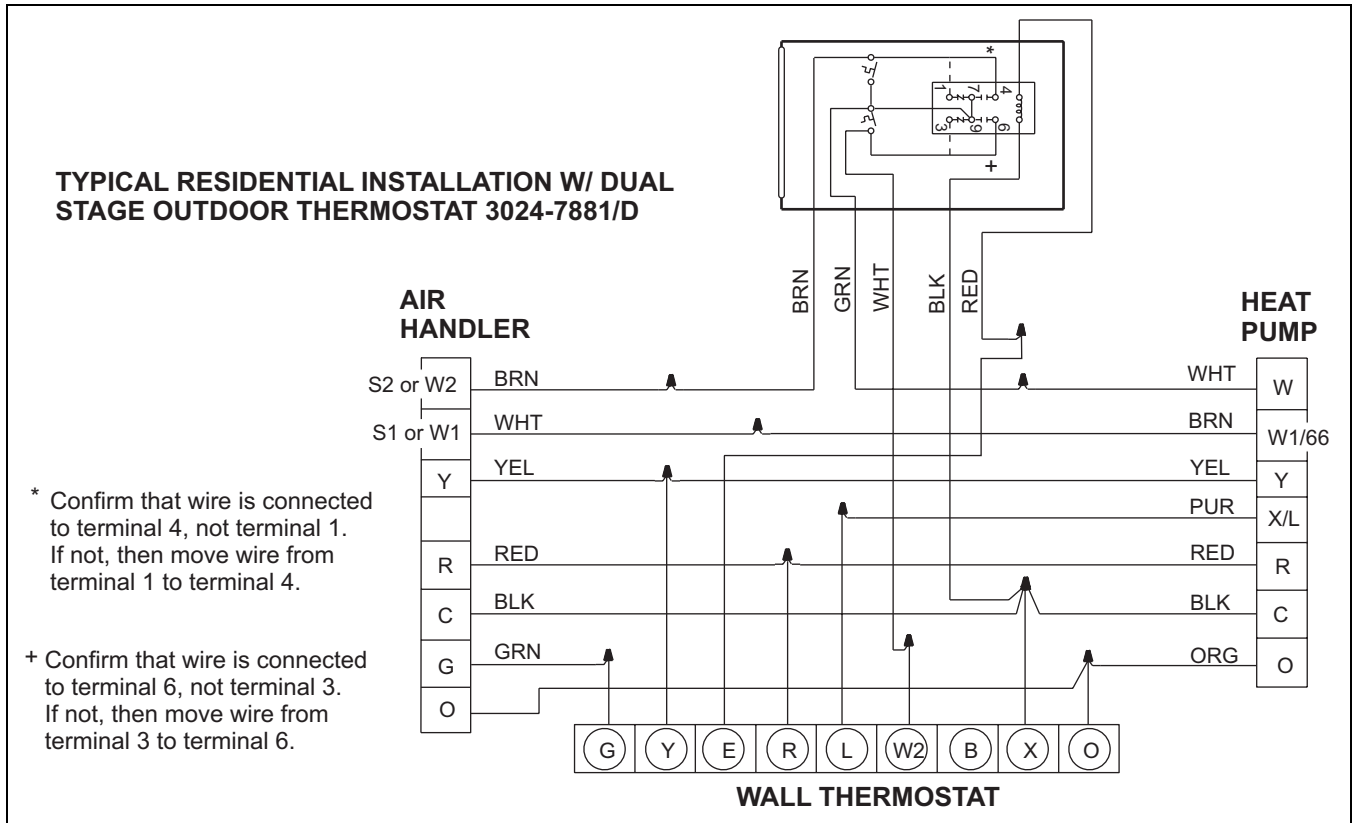
FIGURE 2: Wiring Connections for Typical Residential Installation with Dual Stage Outdoor Thermostat
