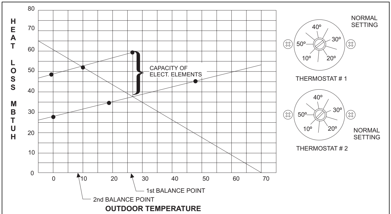
FIGURE 7: Balance Point Determination Chart
