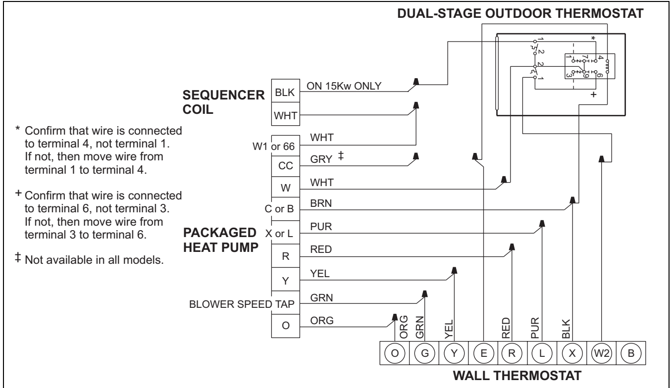
FIGURE 6: Wiring Connections for JP/PHP Packaged Heat Pump with Dual Stage Outdoor Thermostat
