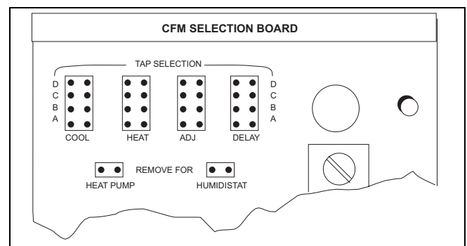
FIGURE 1: CFM Selection Board Detail
