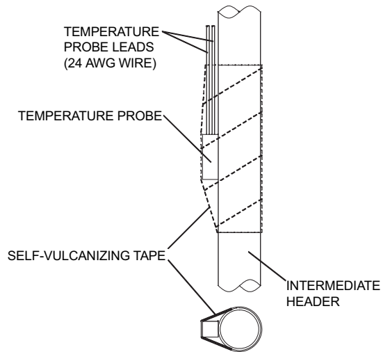
FIGURE 3 - TEMPERATURE PROBE
