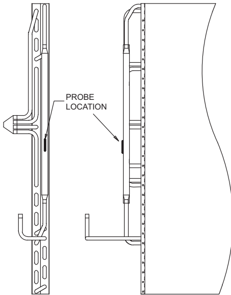
FIGURE 2 - PROBE LOCATION
