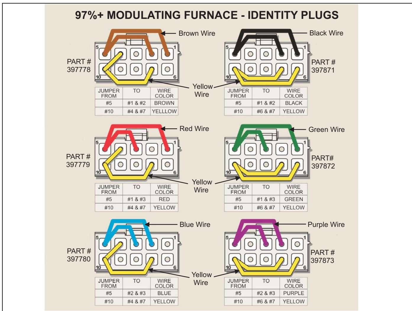
FIGURE 1: 97%+ ID Plug Wire Reference
