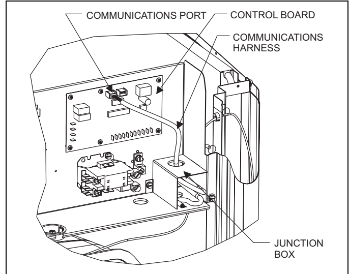
FIGURE 1: Control Box
