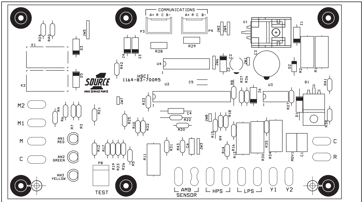
FIGURE 2: AC Communicating Control Module
