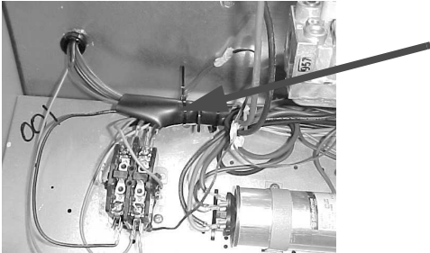
FIGURE 2 - PLASTIC ELECTRICAL TUBE
