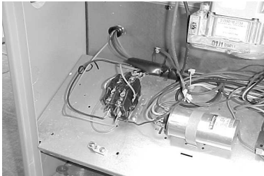
FIGURE 1 - CONTACTOR LOCATION
