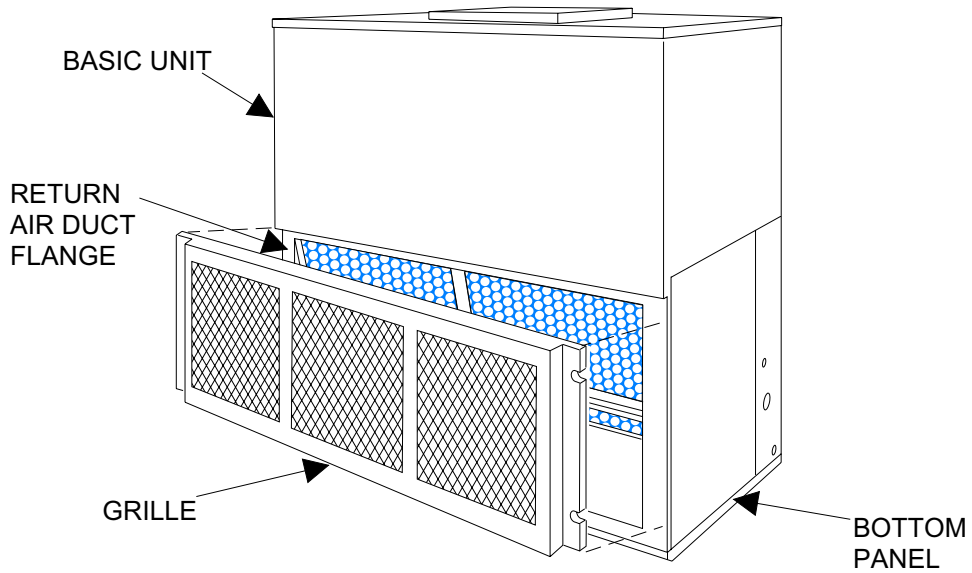
FIGURE 1 - GRILLE ACCESSORY (Typical Installation Vertical Application (Split-System Unit Shown))
