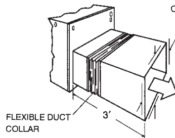
FIGURE 1 - CLEARANCES
