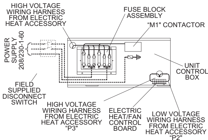
FIGURE 4 - TYPICAL SINGLE POINT 208/230-1-60 FIELD WIRING
