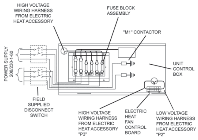
FIGURE 7 - TYPICAL DUAL POINT 208/230-1-60 FIELD WIRING
