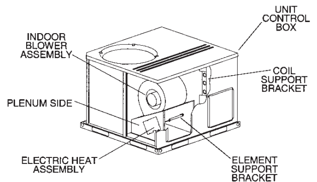
FIGURE 3 - ELECTRIC HEATER MOUNTING
