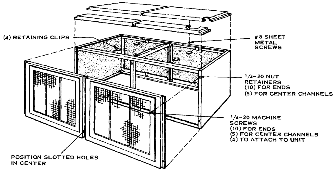
FIGURE 2 - VERTICAL PLENUM ASSEMBLY
