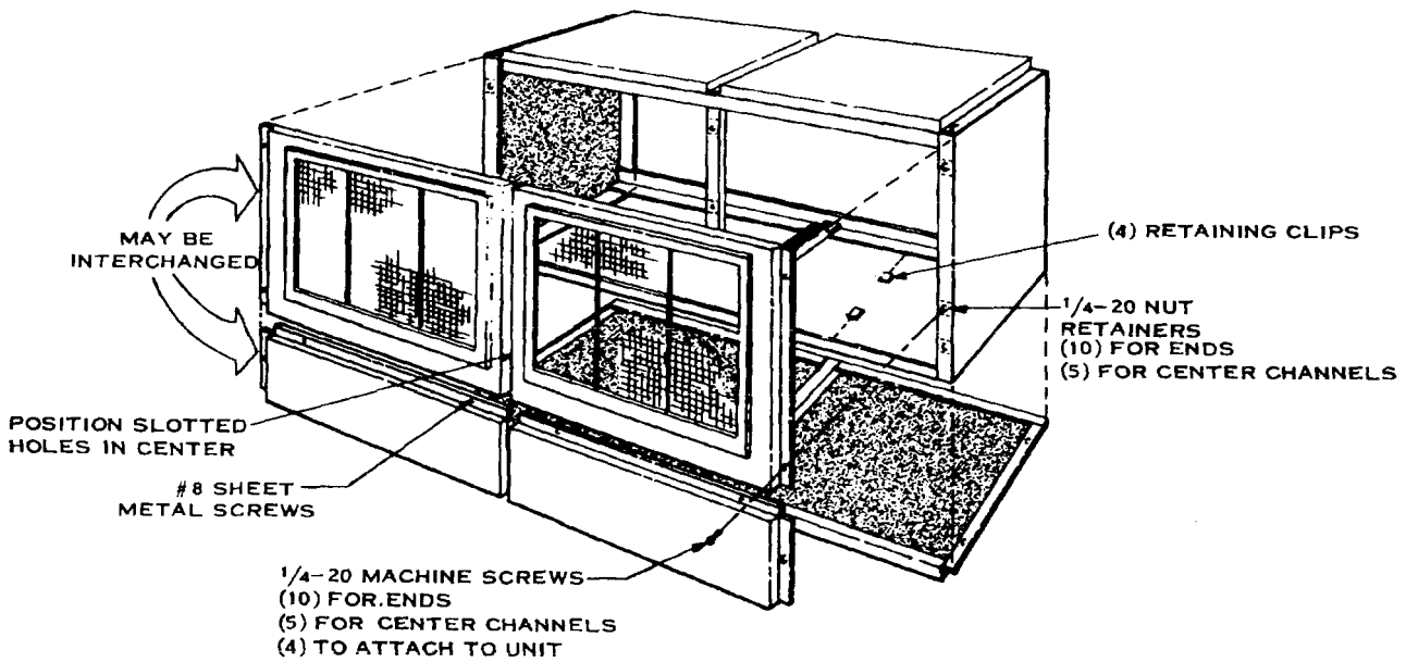
FIGURE 3 - HORIZONTAL PLENUM ASSEMBLY
