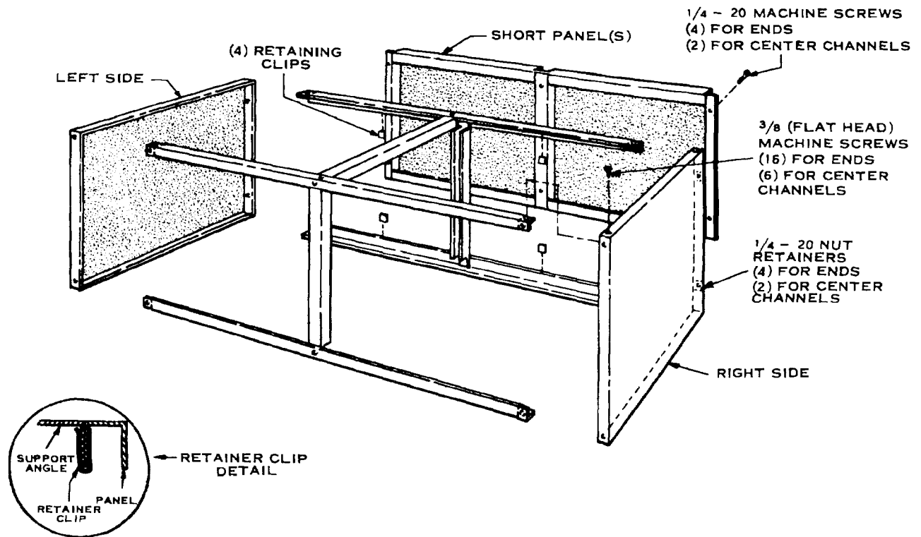
FIGURE 1 - BASIC PLENUM ASSEMBLY
